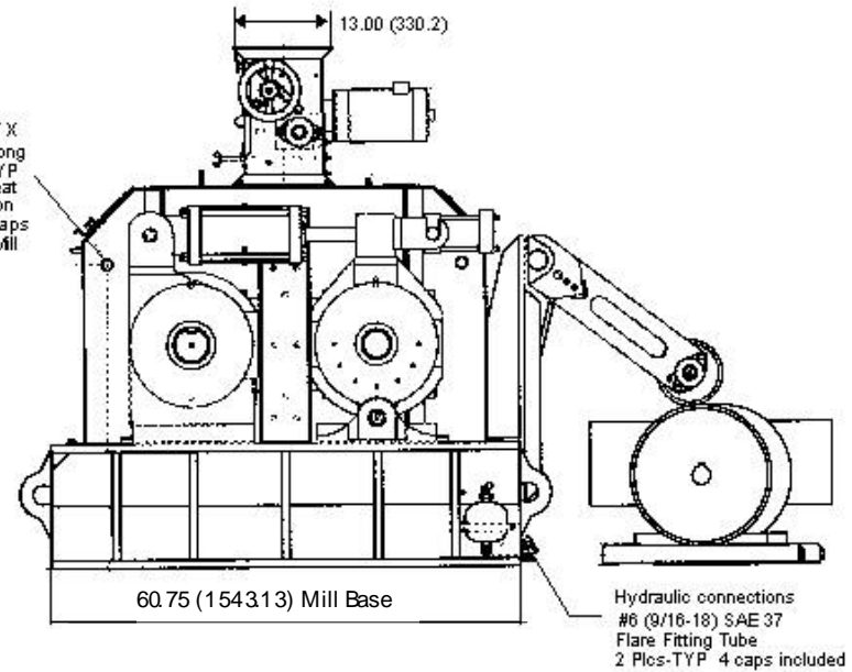
RIGHT SIDE VIEW, GUARDS REMOVED TO SHOW ROLL PREHEAT & HYDRAULIC FITTINGS
